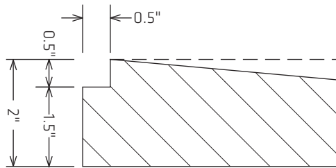
Detail Z' 5x
